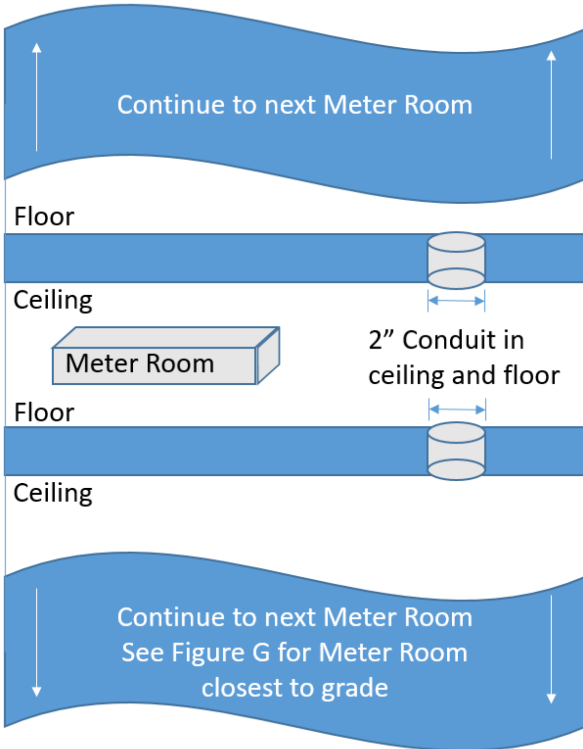
Figure D – Antenna Conduits between Meter Rooms
